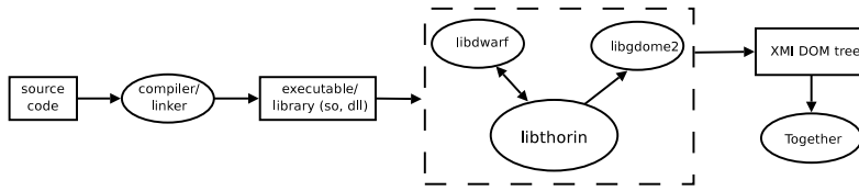
Figure 1: System overview . In this figure we list the important components in libthorin , where the items illustrated inside the dashed rectangle represent our contribution to the system, items to the left of the dashed rectangle represent components that process the application under study in preparation for input to our system and the item to the right of the dashed rectangle represent output of the system.
