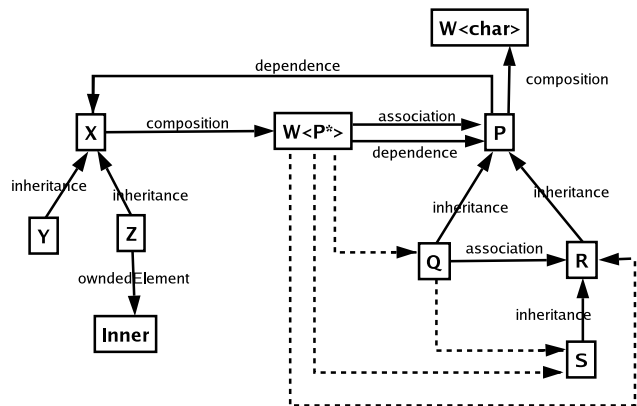
Figure 5. ORD for sample C++ program. This figure illustrates an ORD for the program listed in Figure 4, and the edges that capture relationships between classes in the program. The four dashed lines in the graph are polymorphic edges , and the other edges are labeled appropriately.
