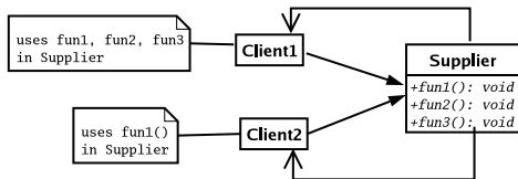
Figure 2. Motivation for stub construction. The UML class diagram in this figure illustrates a cycle of dependencies between a supplier class and two client classes. We use this example to motivate the construction of stubs.
