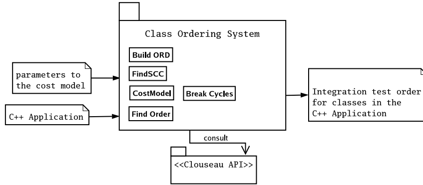
Figure 1. Overview of our Class Ordering System.
