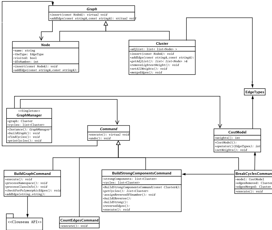
Figure 7. Class Ordering System. This figure illustrates a UML class diagram summarizing the important classes and relationships in our system. The CostModel class in the middle right of the figure encapsulates our parameterized cost model. There is a cycle in the class diagram that includes classes Graph , Node and Cluster .
