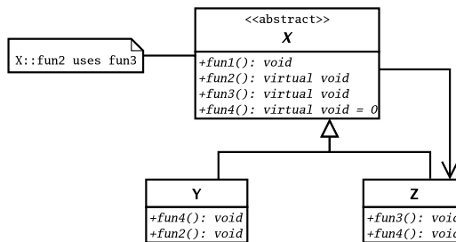
Figure 3. Stub for an abstract base class. The UML class diagram in this figure illustrates an abstract base class and two derived classes that override some of the functions in the base class. We use this example to describe the difficulty of stub construction for abstract base classes.
