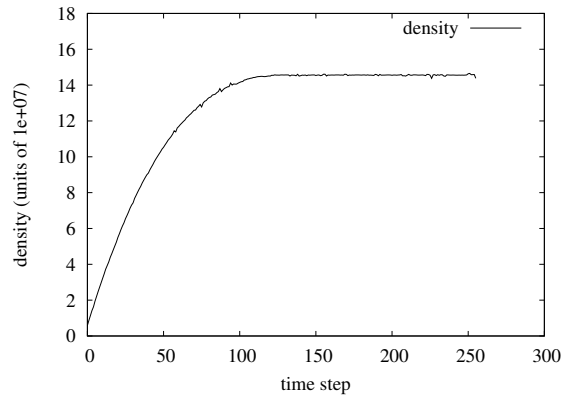
Figure 5: The total density in the lattice at each time step for the 128x128x128 lattice shown in Figure 2
