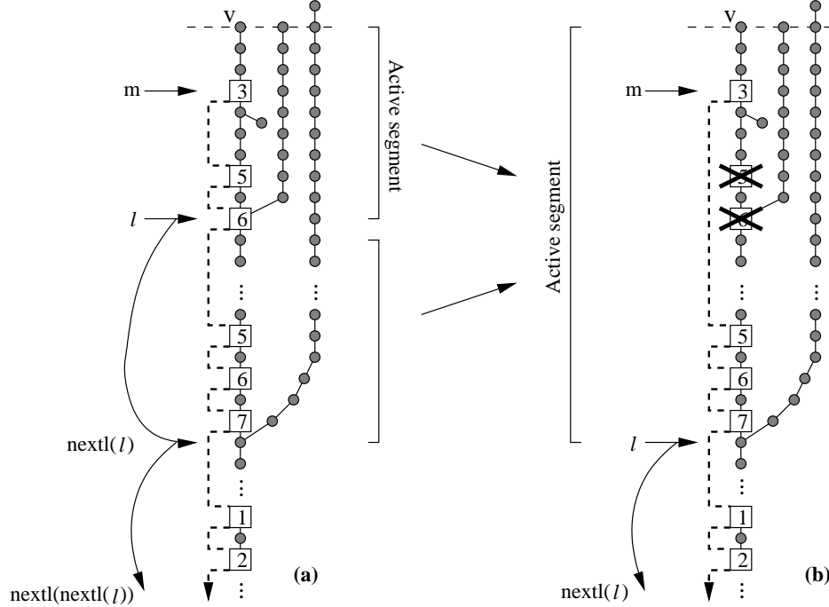
Figure 4: Illustrations of (a) an m -list (drawn with dotted links), and (b) the operation of splicing together the portions of the m -list belonging to the top two segments of the l -list. This event happens whenever v “escapes” from the current upward overhang from l (upward overhangs are emphasized in the figure by stretching these paths upward). The other m -list of different parity is not pictured, but it would also be spliced in the same fashion. The boxed number shown at a vertex x is val(x) .
