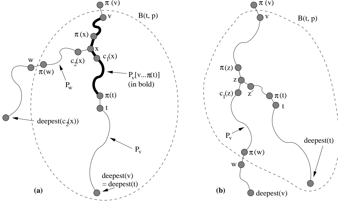
Figure 1: Searching for vertices in N(t, p) .
