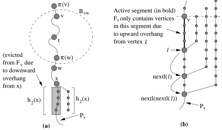
Figure 3: Illustration of the downward and upward overhang conditions. In (a), the downward overhang of length h_2(x) branching off x permanently disqualifies the h_2(x) vertices in its “shadow” below x on P_v from belonging to F_v . In (b), the upward overhang from l (actually a downward path that branches off and descends from l , which we visualize by stretching it out upward) prevents any choice of w below l from belonging to F_v . When our algorithm steps from v to \pi(v) , we will “escape” from this upward overhang and be constrained instead by the larger upward overhang branching off nextl(l) . The current stack of nested upward overhangs branching off l , nextl(l) , and so on, forms what we call the l -list.
